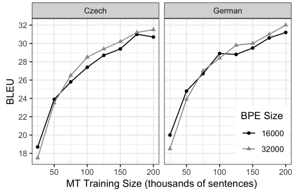
Figure 1: MT test BLEU for all training configurations.
